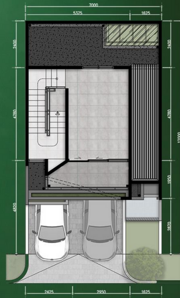
Denah Lantai 3
