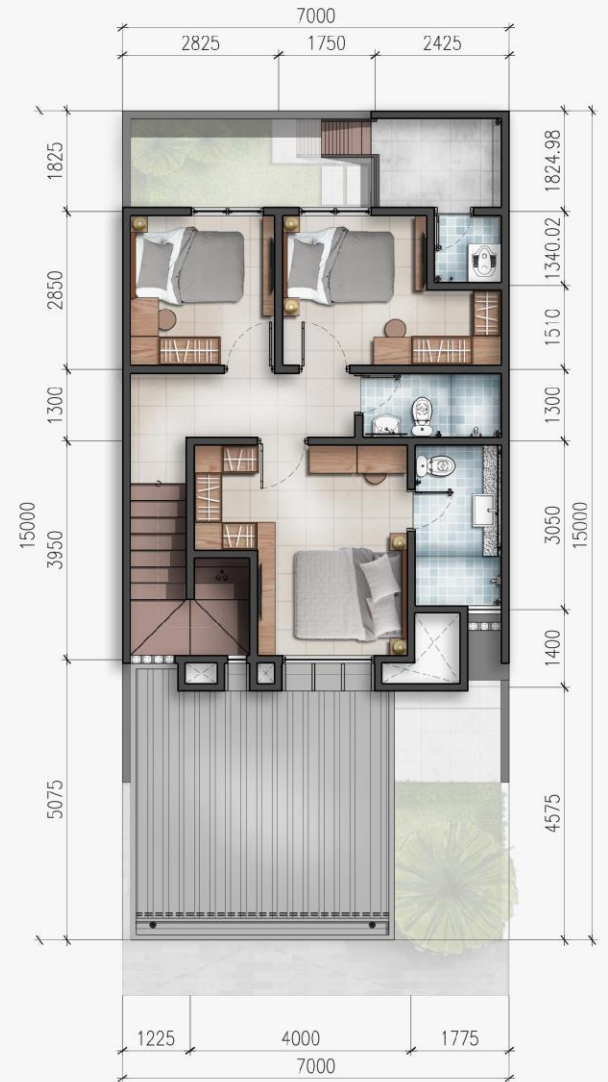
DENAH LT. 2
